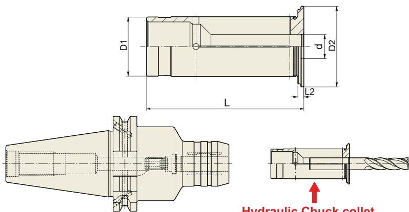
Hydraulic Chuck collet
